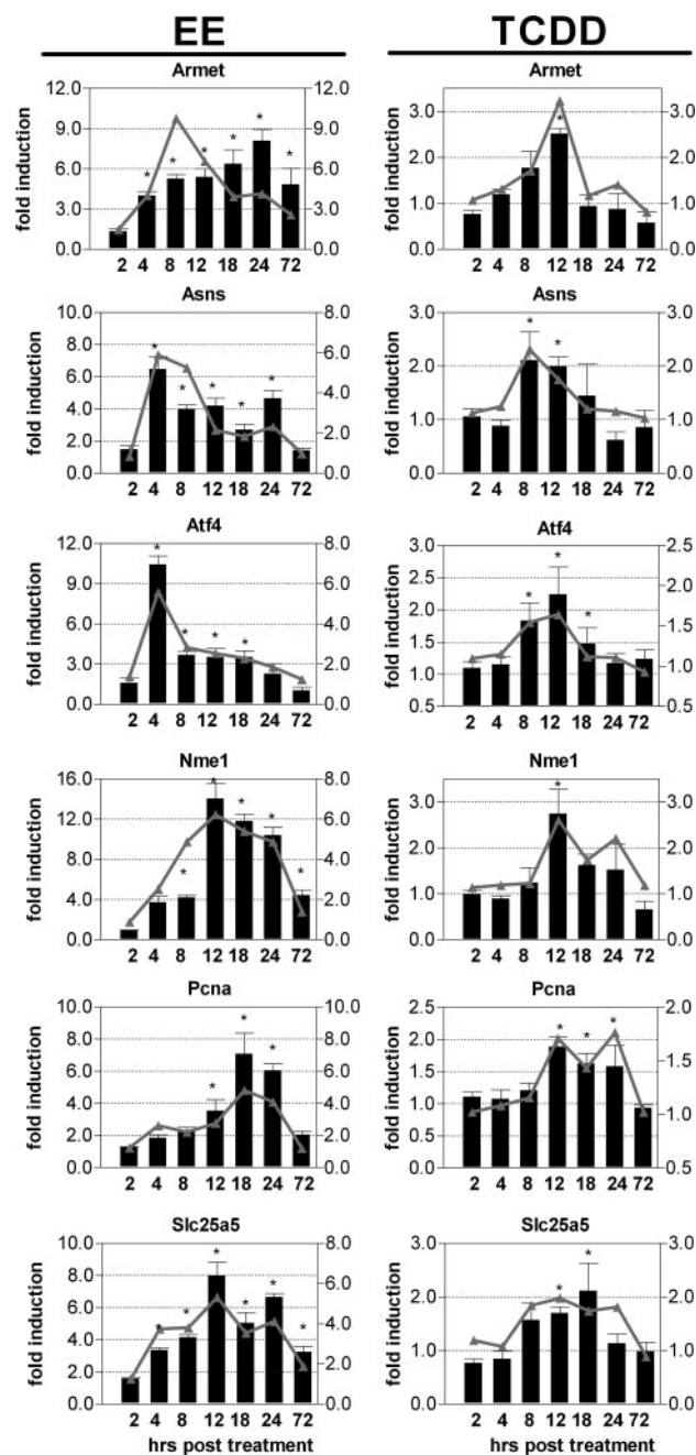
Fig. 2. Quantitative real-time PCR verification of temporal microarray results. The same RNA used for cDNA microarray analysis was examined by QRT-PCR. All fold changes were calculated relative to time-matched vehicle controls. Bars (left axis) and lines (right axis) represent data obtained by QRT-PCR and cDNA microarrays, respectively, whereas the x-axis represents the time points. Genes are indicated by official gene symbols and results are the average of five biological replicates. Error bars represent the S.E.M. for the average fold change. *, p < 0.05 for QRT-PCR.
