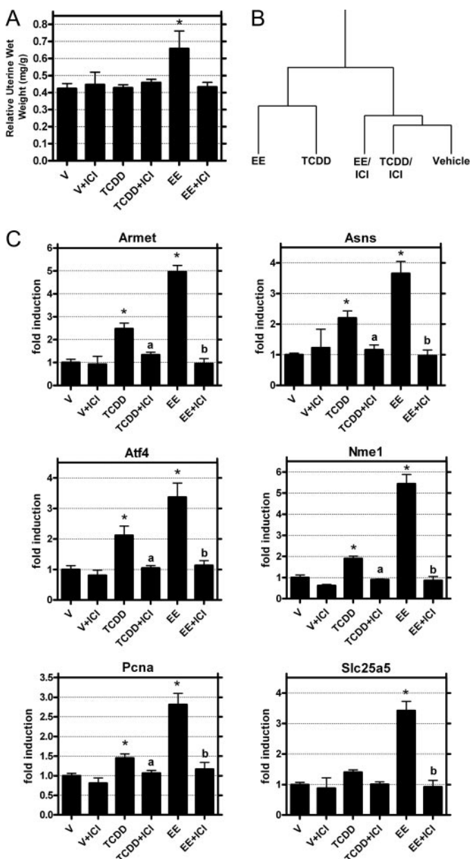
Fig. 3. ICI 182 780 inhibits uterine gene expression responses to TCDD. A, uterine wet weights for each treatment group at 12 h. B, hierarchical clustering of the normalized intensity values from the microarrays illustrates that the EE and TCDD treatment groups cluster together whereas the EE/ICI and TCDD/ICI groups cluster with the vehicle control. C, QRT-PCR was used to examine gene expression responses to EE and TCDD in the absence and presence of the pure ER antagonist ICI 182 780. All -fold changes were calculated relative to time-matched vehicle controls. Genes are indicated by official gene symbols and results are the average of six biological replicates. Error bars represent the S.E.M. for the average -fold change. *, p < 0.05 compared with vehicle control; a, p < 0.05 for ICI/TCDD mice compared with TCDD-treated mice; b, p < 0.05 for ICI/EE mice compared with EE-treated mice.
