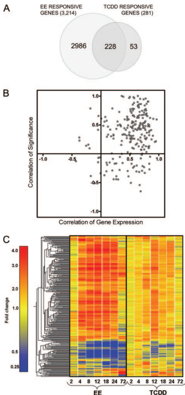
Fig. 1. Overlap of active uterine gene expression responses from temporal TCDD and EE studies. A, 3214 and 281 unique genes were identified as differentially expressed at one or more time points in the EE and TCDD studies, respectively. Of these genes, 228 were responsive in both studies. B, correlation analysis of temporal gene expression and significance. The majority of the genes fall into the upper right quadrant, identifying genes that are highly correlated between both gene expression and significance. A number of genes also fall into the lower right quadrant, which represents genes with high correlation of expression but a lower correlation of significance. These results indicate that the temporal patterns of TCDD-induced gene expression responses are similar to those elicited by EE. C, gene-based hierarchical clustering reveals the similarity of the EE and TCDD gene expression profiles while also illustrating the lower magnitude of change in response to TCDD.
